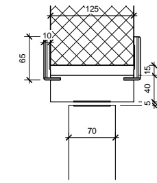
3 Head Detail 1 : 5
