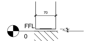
4 Undercut Detail 1 : 5
