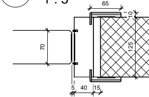
4 Undercut Detail 1 : 5
